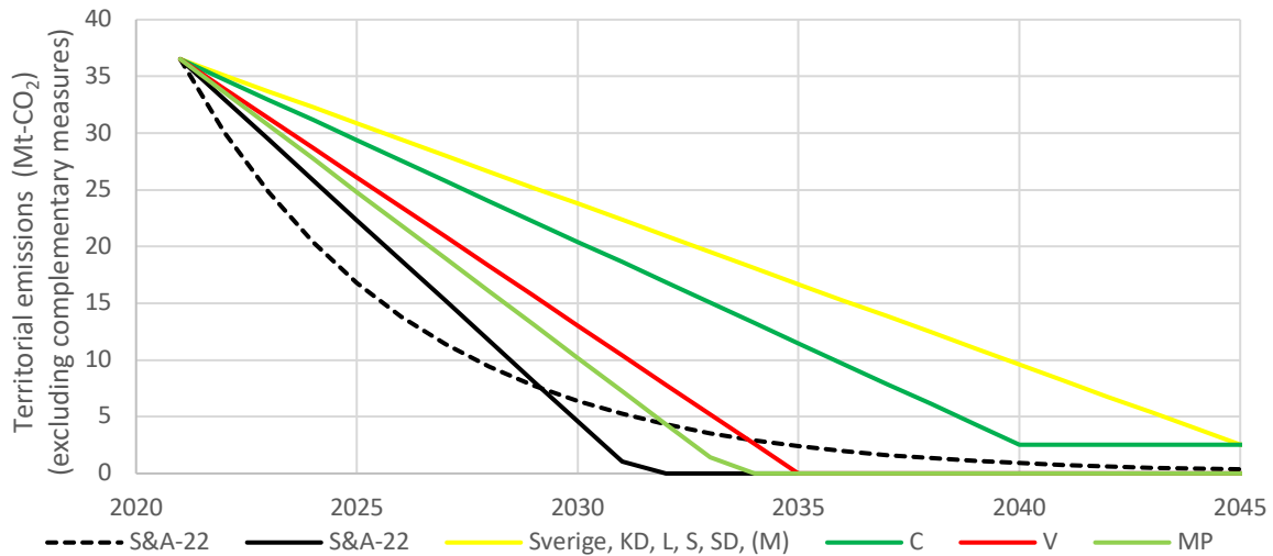
Figure 4. Comparison of parties' ambitions for linear emissions reductions in Mton-CO 2 (carbon dioxide only) for fossil fuels and industry (excluding international travel) excluding complementary measures with Sweden's current target (yellow line) and exponential (dashed black line) and linear (solid black line) climate just trajectories (S&A-22). Note that this is a hypothetical "end-member" scenario in which parties are assumed to follow linear trajectories to a baseline of 2.5 Mton-CO 2 in 2045 (Naturvårdsverket, 2021). Also, no attempt has been made to assess the feasibility of parties' stated ambitions.
