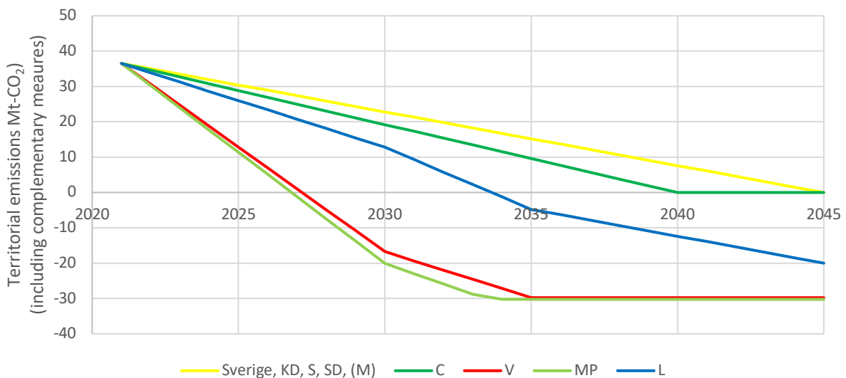
Figure 5. Comparison of parties' ambitions for linear emissions reductions in Mton-CO 2 (carbon dioxide only) for fossil fuels and industry (excluding international travel) including complementary measures with Sweden's current target (yellow line). Note that this is a hypothetical "end-member" scenario in which parties are assumed to follow linear trajectories. Also, no attempt has been made to assess the feasibility of parties' stated ambitions.
