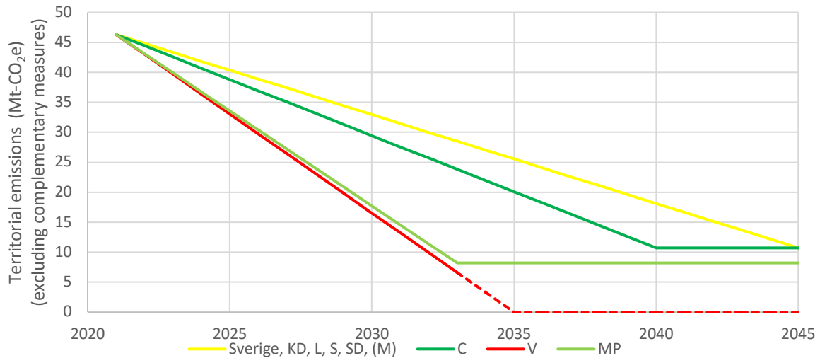
Figure 2. Comparison of parties' ambitions for emissions reductions in Mton-CO 2 e (carbon dioxide and other greenhouse gases), assuming linearity, excluding complementary measures with Sweden's current target. Note: V's stated ambition is "real zero" for CO 2 e. It is unclear if this can be achieved for all non-CO 2 emissions. If not, V's trajectory will be similar to MP's trajectory. Note that these are hypothetical trajectories because no attempt has been made to assess the feasibility of parties' stated ambitions.
