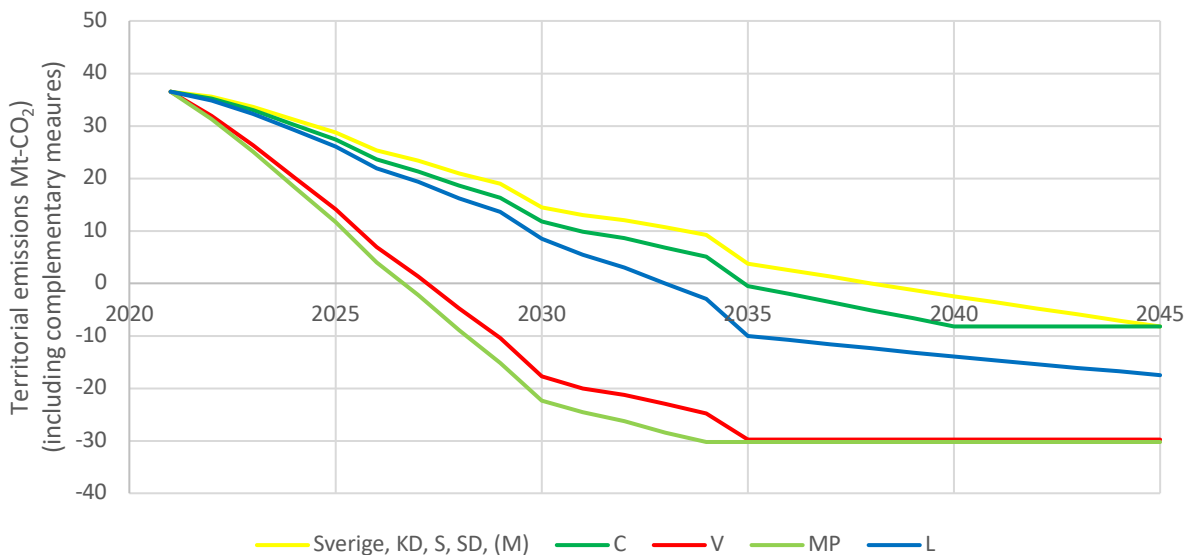
Figure 7. Comparison of parties' ambitions for emissions reductions in Mton-CO 2 (carbon dioxide only) for fossil fuels and industry (excluding international travel), including complementary measures with Sweden's current target (yellow line). Note that this is a hypothetical "end-member" scenario in which parties are assumed to follow trajectories similar to Scenario 2021/80 (Naturvårdsverket, 2021). Also, no attempt has been made to assess the feasibility of parties' stated ambitions.
