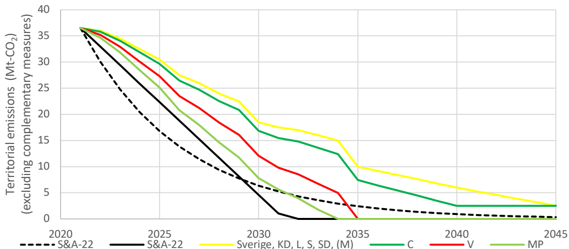
Figure 6. Comparison of parties' ambitions for emissions reductions in Mton-CO 2 (carbon dioxide only) for fossil fuels and industry (excluding international travel), excluding complementary measures with Sweden's current target (yellow line) and exponential (dashed black line) and linear (solid black line) climate just trajectories. Note that this is a hypothetical "end-member" scenario in which parties are assumed to follow trajectories similar to Scenario 2021/80 (Naturvårdsverket, 2021). Also, no attempt has been made to assess the feasibility of parties' stated ambitions.
