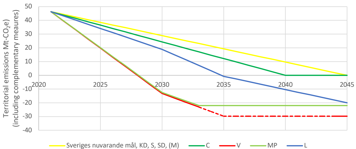
Figure 3. Comparison of parties' ambitions for emissions reductions in Mton-CO 2 e (carbon dioxide and other greenhouse gases), assuming linearity, including complementary measures with Sweden's current target. Note: V's stated ambition is "real zero" for CO 2 e. It is unclear if this can be achieved for all non-CO 2 emissions. If not, V's trajectory will be similar to MP's trajectory. Note that these are hypothetical trajectories because (with the exception of the aforementioned concern) no attempt has been made to assess the feasibility of parties' stated ambitions.
